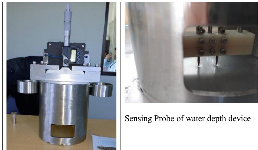
Figure 6. Measuring device after assembled
